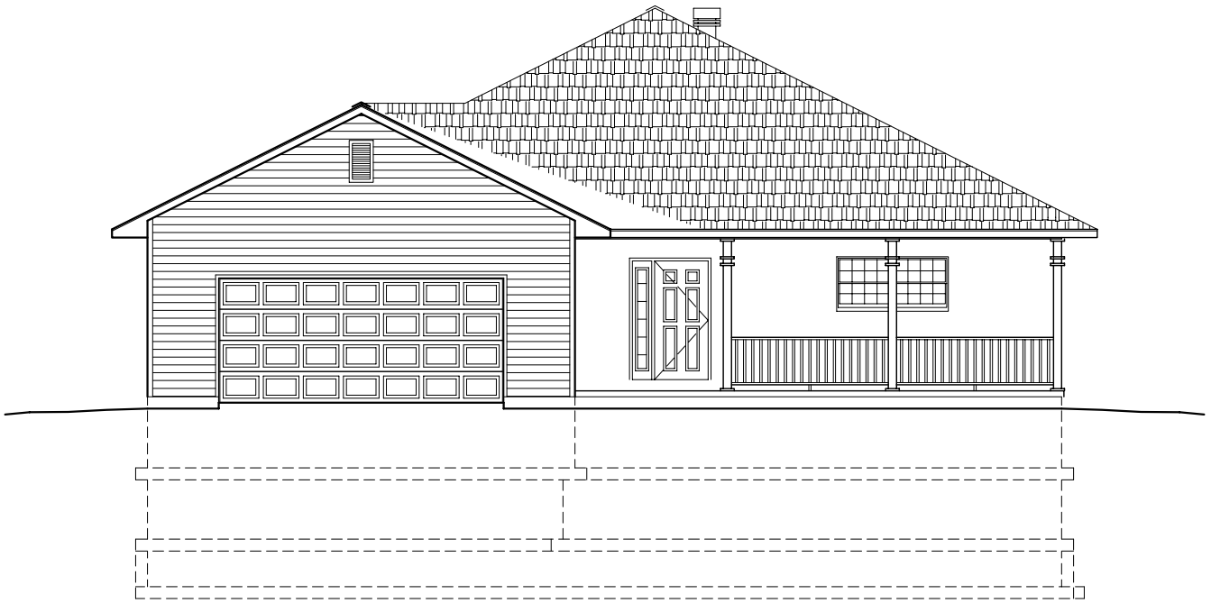
1 FRONT ELEVATION A-1
